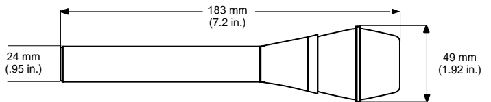
OVERALL DIMENSIONS FIGURE 5
