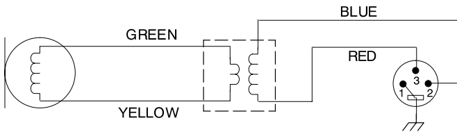
INTERNAL WIRING
