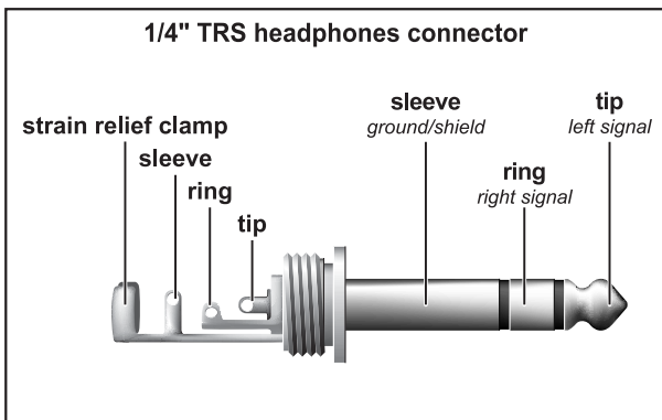
Fig. 8.4: Headphones connector
