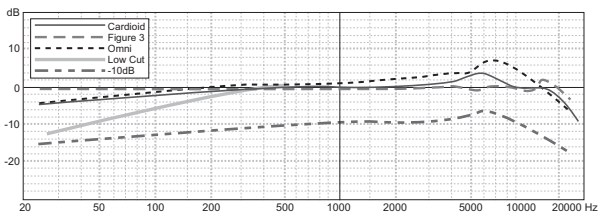
Frequency response
