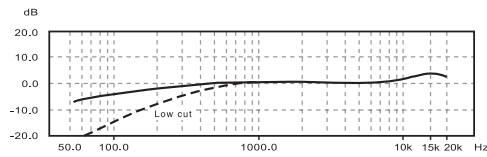
Frequency response (cardioid)
