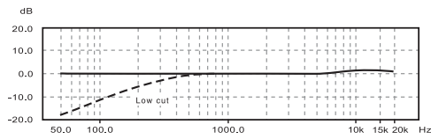
Frequency response (omnidirectional)
