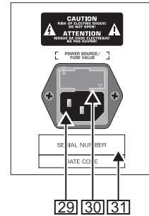
Fig. 2.3: Standard IEC power receptacle, fuse holder and serial number (rear panel)
