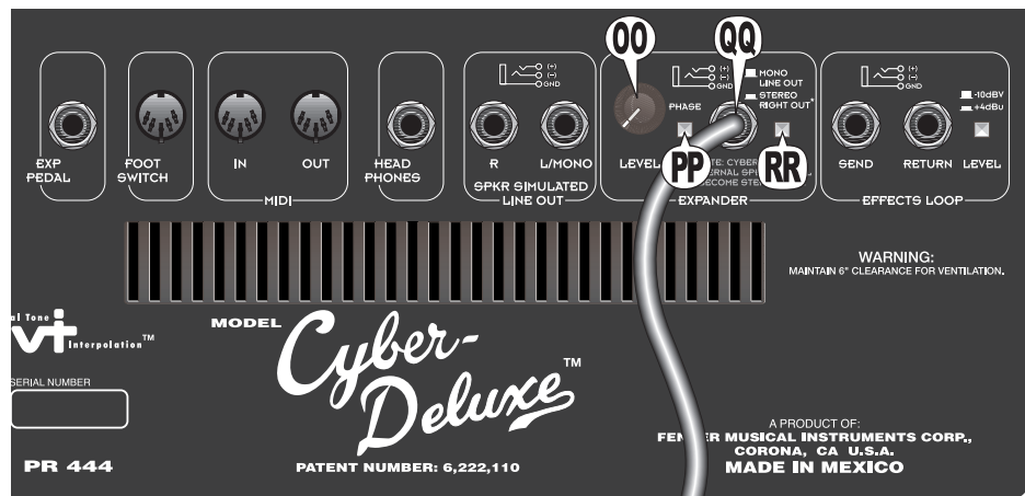
Figure 3a Stereo Expander Connection
