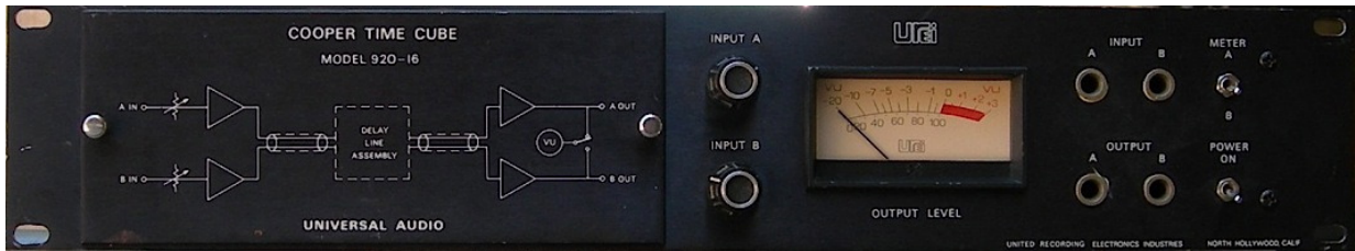
Figure 28. The original Cooper Time Cube hardware front panel
