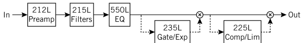
Figure 10. PREDYN routes the 550L before the dynamics modules
