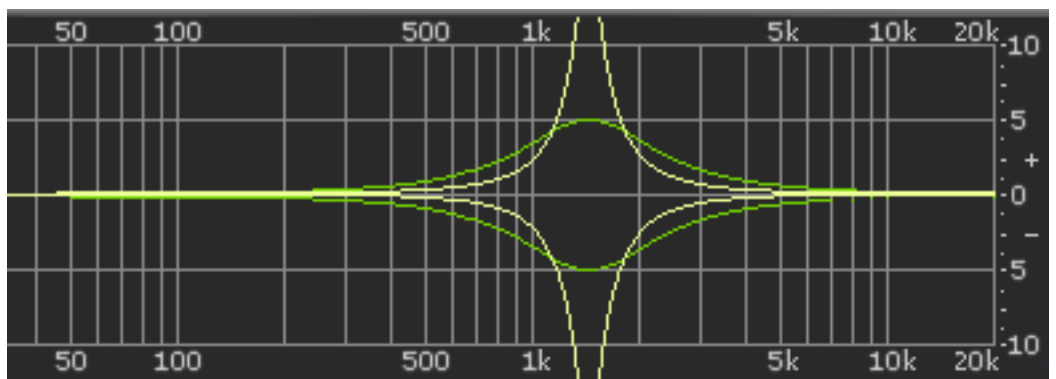
Figure 21. Parametric Type III response
