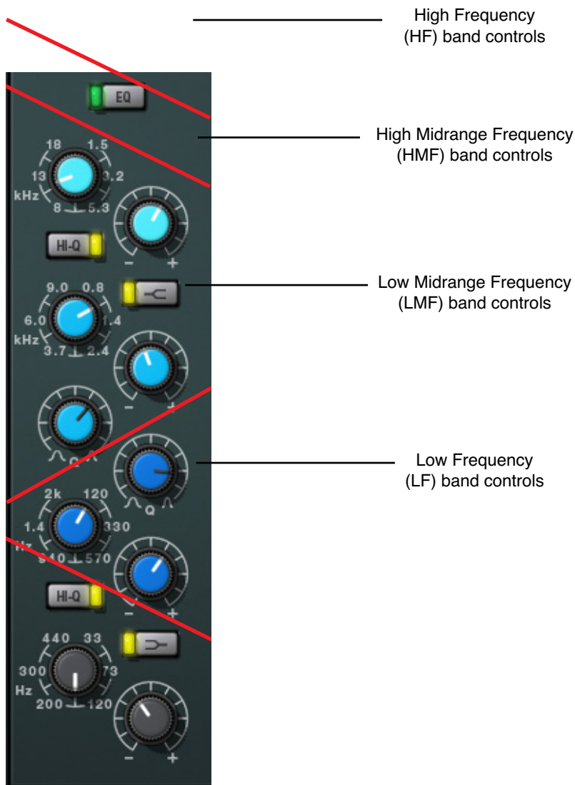
Figure 86. Neve 88RS EQ Controls Layout
