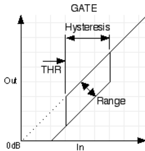
Figure 85. Hysteresis in the Neve 88RS Gate
