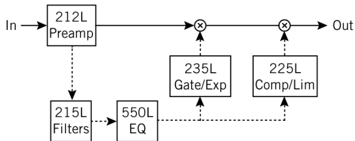
Figure 13. Signal flow with SC enabled in both 215L and 550L modules
