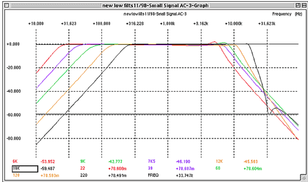
Figure 68. High Pass and Low Pass filter response curves (standard version)
