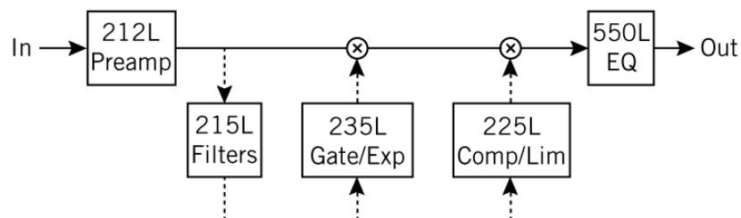
Figure 8. Simplified signal flow illustrating parallel side chain inputs with 215L SC enabled
