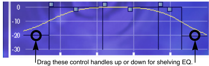
Figure 39. DreamVerb Resonance Shelving Bands
