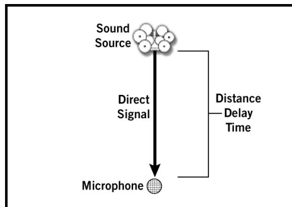
Figure 90. Illustration of Distance Delay. When set to aligned, this “extra” time is eliminated.
