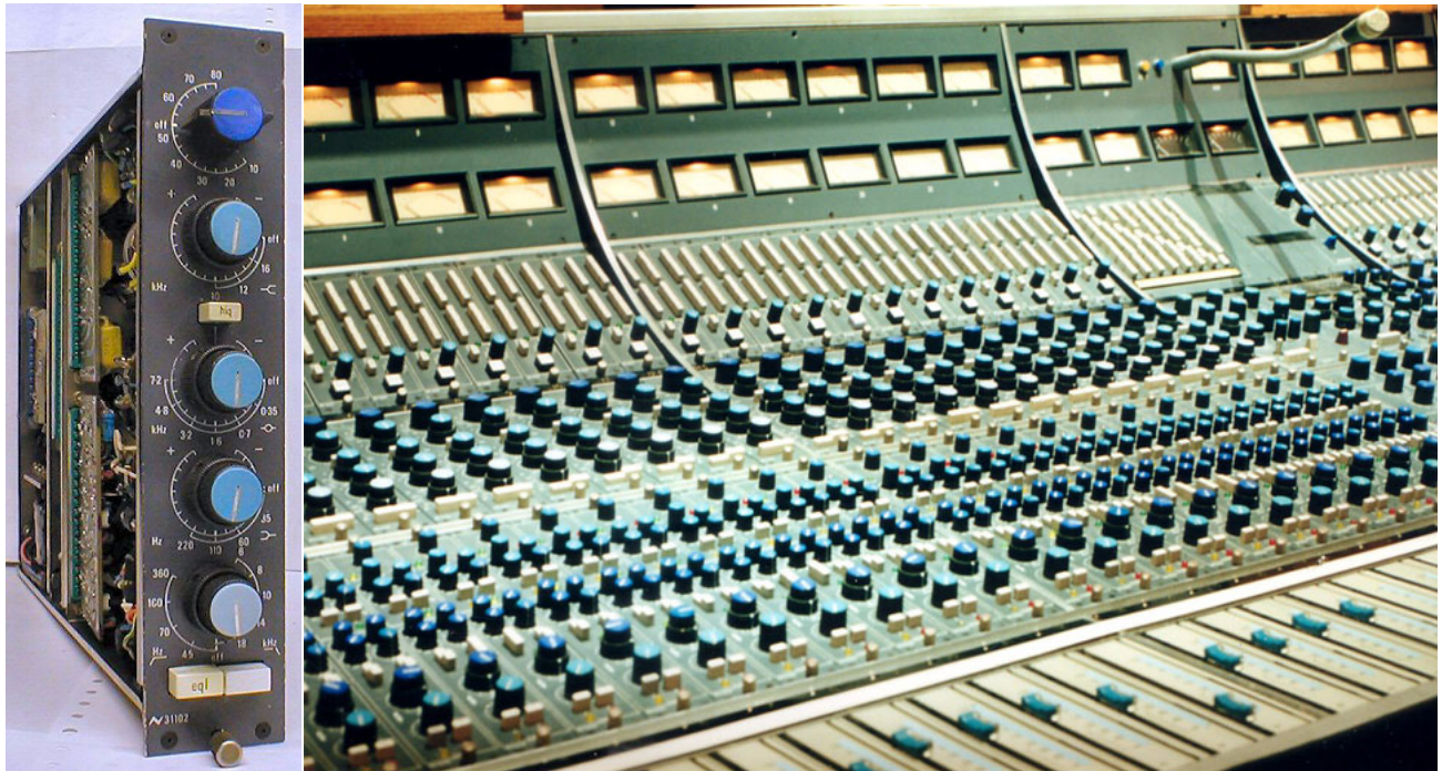
One Neve 31102 EQ hardware module and 31102s installed in a Neve 8068 console
