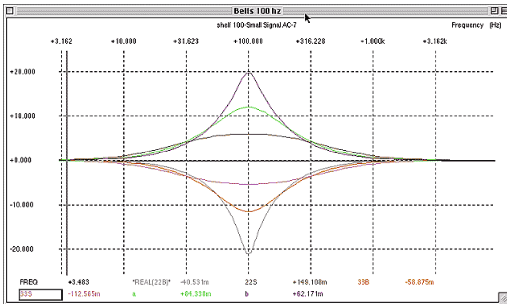
Figure 66. Effect of Bandwidth control on response curve in Bell mode
