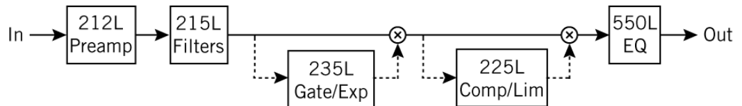
Figure 7. Simplified default signal flow within the API Vision Console Channel Strip
