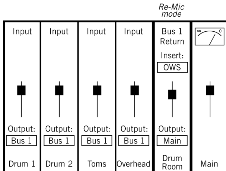
Figure 92. DAW signal routing with OWS in Re-Mic mode on a drum submix
