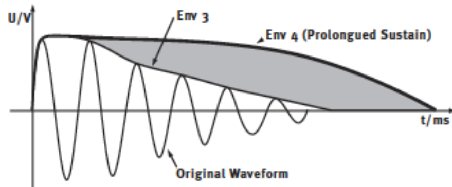
Figure 136. SPL Transient Designer Sustain Envelopes
