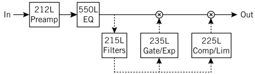
Figure 11. The 550L always precedes the side chain tap when PREDYN is active
