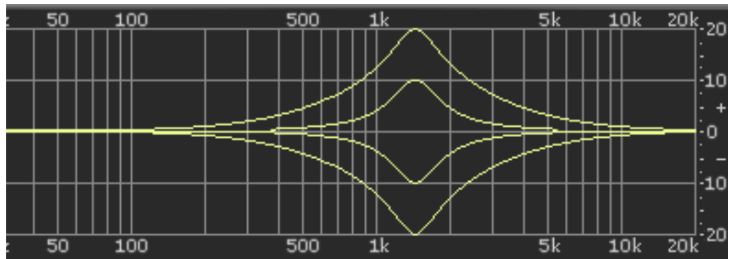
Figure 19. Parametric Type I response
