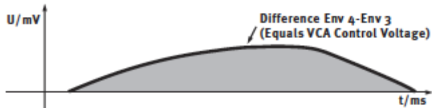
Figure 137. SPL Transient Designer Sustain Control Voltage
