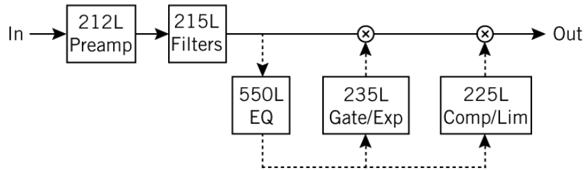
Figure 12. Signal flow with 550L SC enabled
