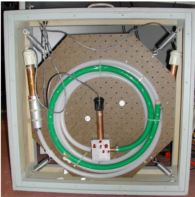
Figure 29. The opened acoustic module and the complete system
