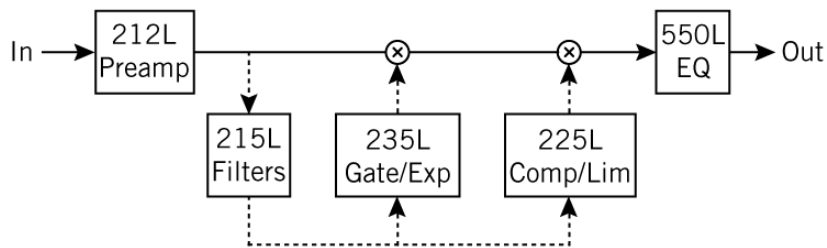
Figure 9. Signal flow with 215L Sweep Filters SC enabled
