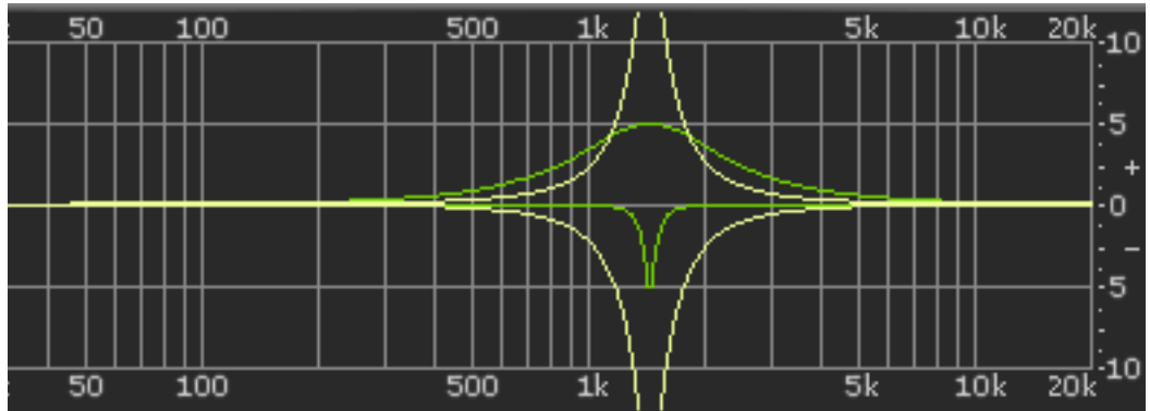
Figure 20. Parametric Type II response
