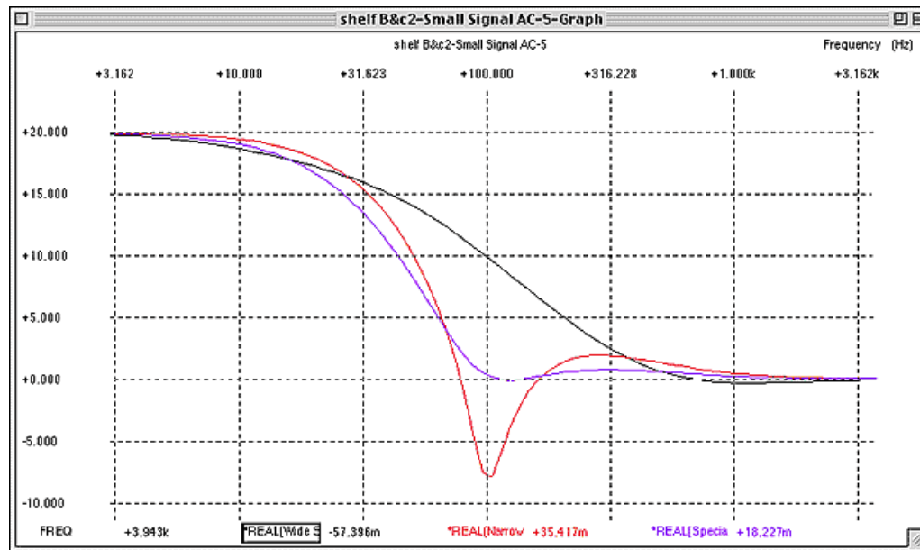
Figure 67. Effect of Bandwidth control on response curve in Shelf mode
