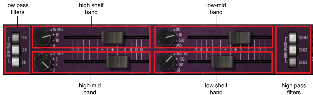
Figure 149. Trident A-Range band control layout
