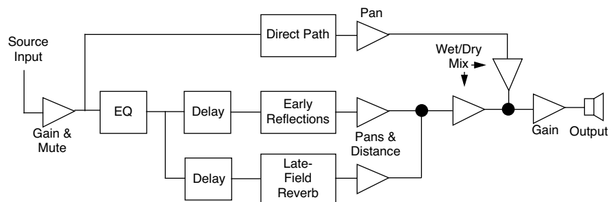
Figure 37. DreamVerb signal flow
