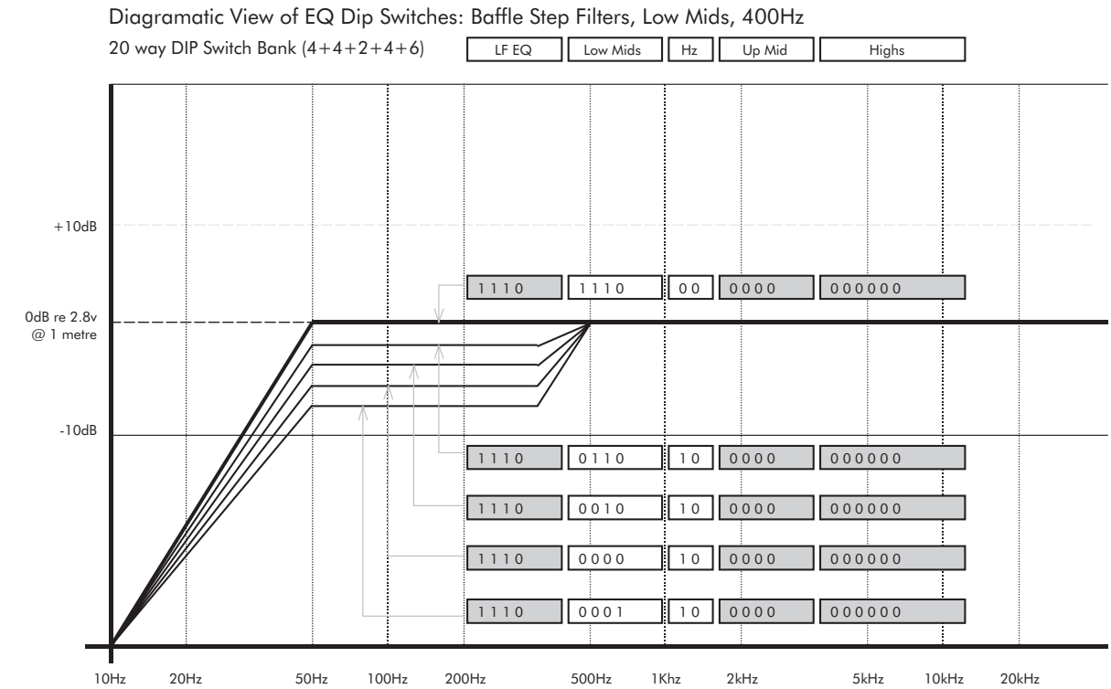
Fig. 4. DIP switches 5 to 8 control amplitude, 9 & 10 control frequency - set here to 400Hz. All other DIPs set to 'flat'.
