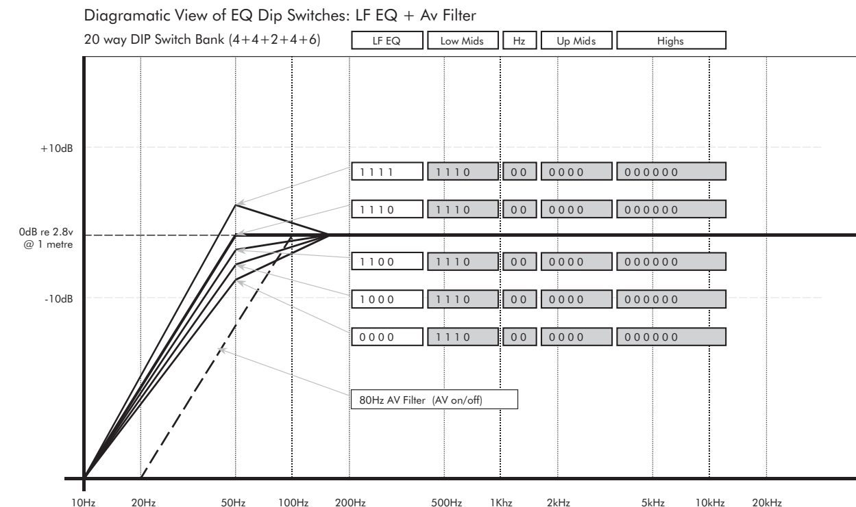
Fig. 2. Range of adjustment available and settings for the first 4 DIP switches. All other DIPs set to 'Flat'
