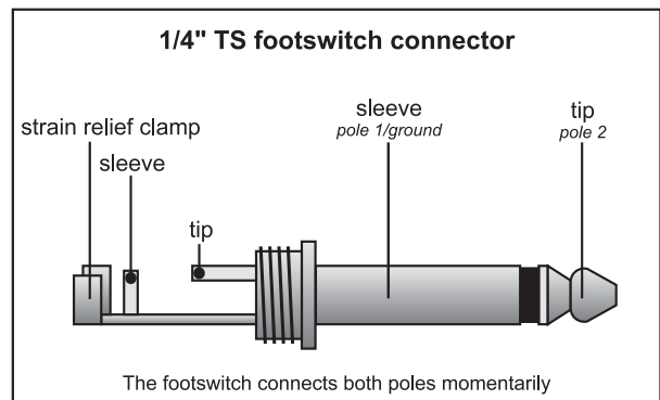
Fig. 9.3: Footswitch connector
