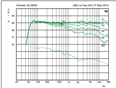
Figure 6. The curves show the horizontal directivity characteristics of the M030. The lower curve shows the loudspeaker's power response.
