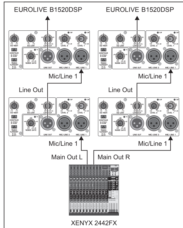
Fig. 4.3: Linking several B1520DSP speakers
