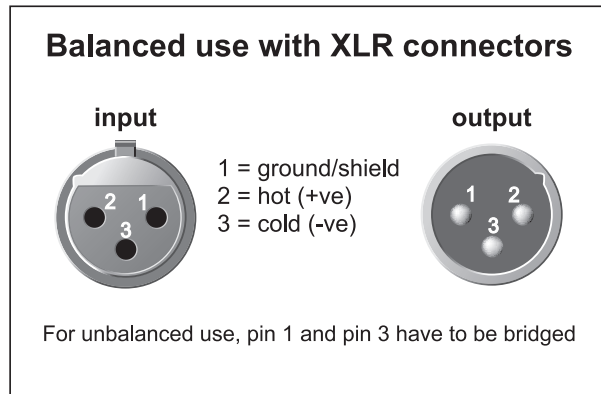
Fig. 5.1: XLR connector
