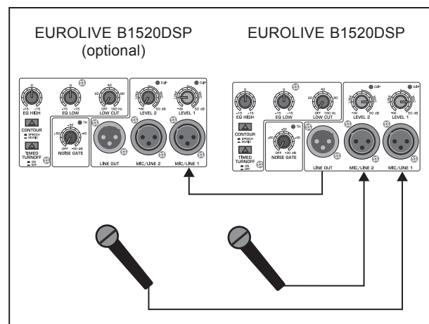
Fig. 4.1: Connecting microphones
