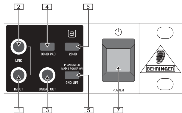
Fig. 2.1: Front panel control elements
