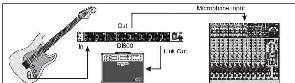
Fig. 3.1: Guitar → DI-box → guitar amp/mixer
