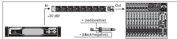
Fig. 3.4: Connection to a power amp output
