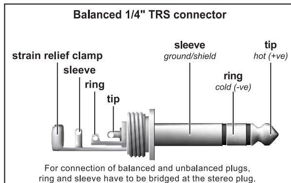
Fig. 4.3: 1/4" TRS connector
