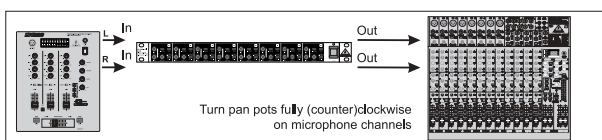
Fig. 3.2: DJ mixer → DI-box → mixer
