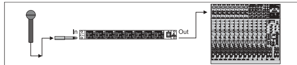
Fig. 3.3: Microphone connection
