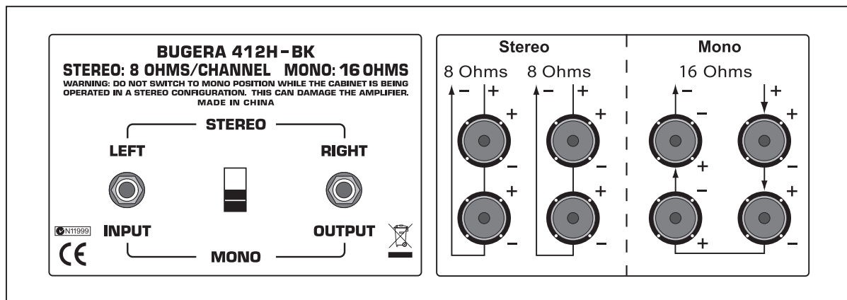
Rear panel
