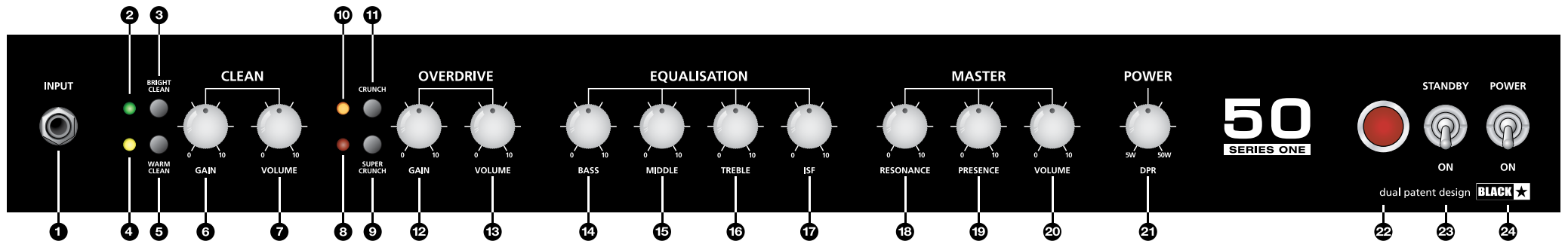
Front Panel
