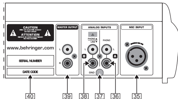
Fig. 3.2: The rear-panel audio connectors of the BCD3000
