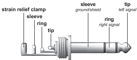
Fig. 7.2: 1/4" TRS headphones connector
